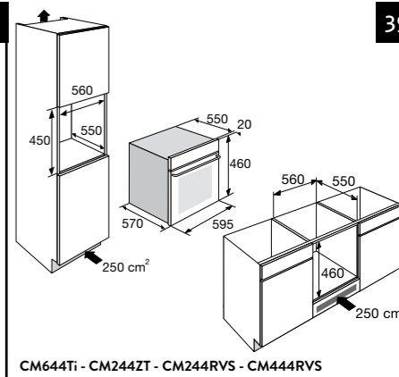
CM644Ti - CM244ZT - CM244RVS - CM444RVS
